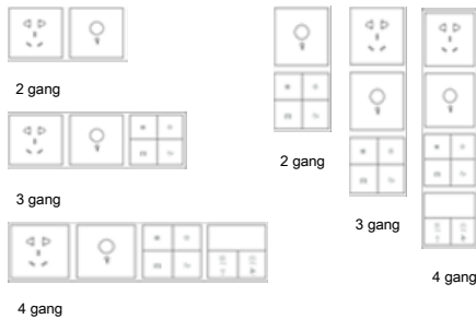
Figure 12. Horizontal installation
