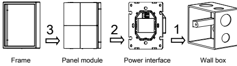
Figure 11. Installation
